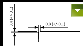
2mV – microchanfrein
