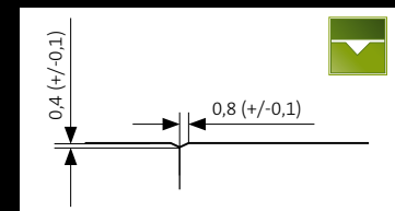
2mV – micro bevel
