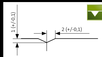
2V – standard bevel
